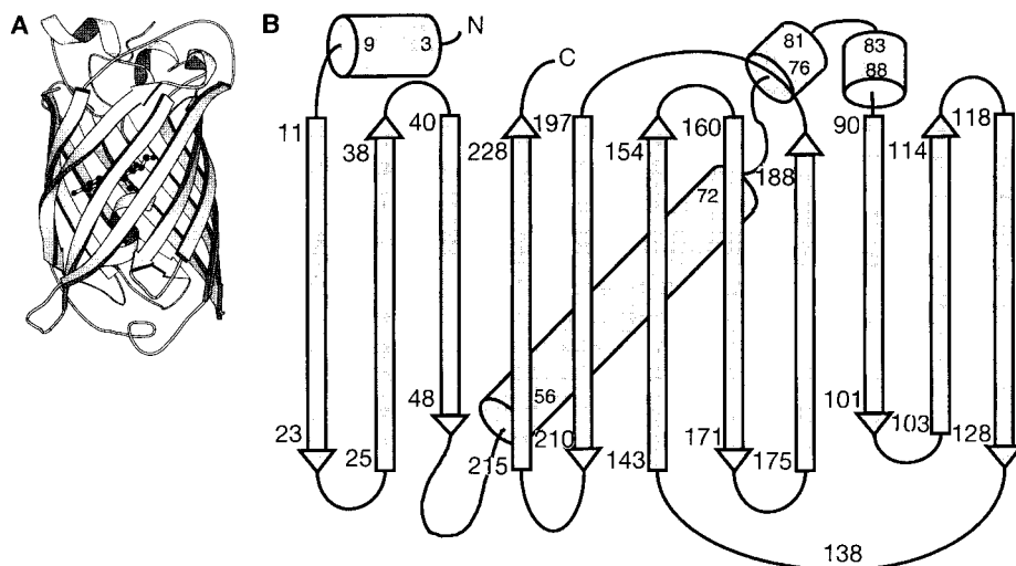
Fig. 1. (A) Schematic drawing of the backbone of GFP produced by the program MOLSCRIPT (32). The chromophore is shown as a ball and stick model. (B) Schematic drawing of the overall fold of GFP. Approximate residue numbers mark the beginning and ending of the secondary structure elements. N, NH 2 -terminus; C, COOH-terminus.
